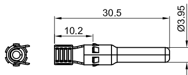
Male Contact
