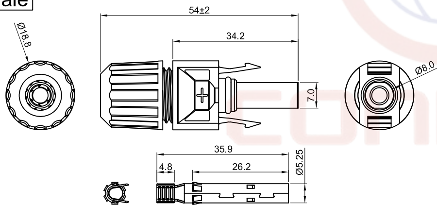
Female Contact
